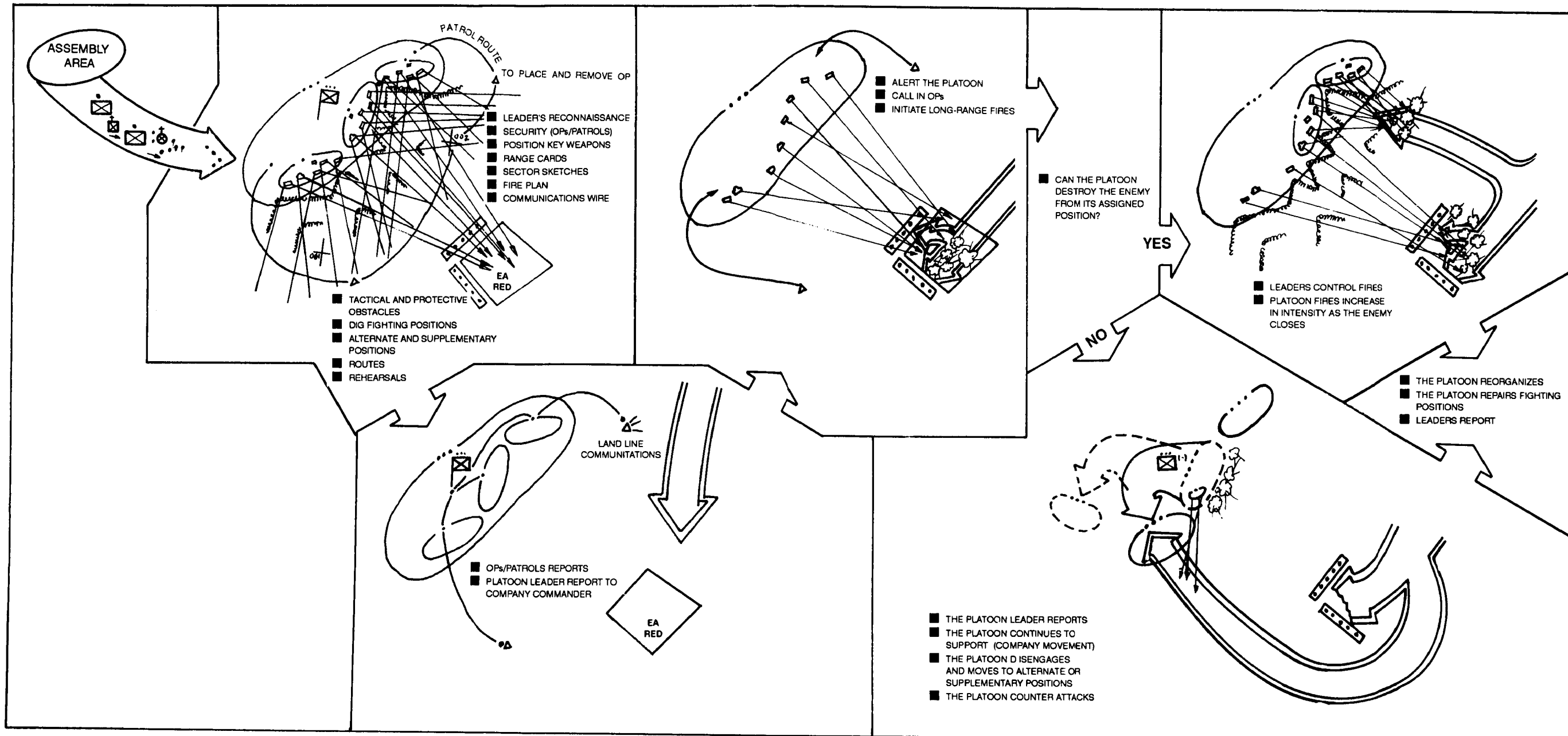
Figure 2-36. Platoon defend.
